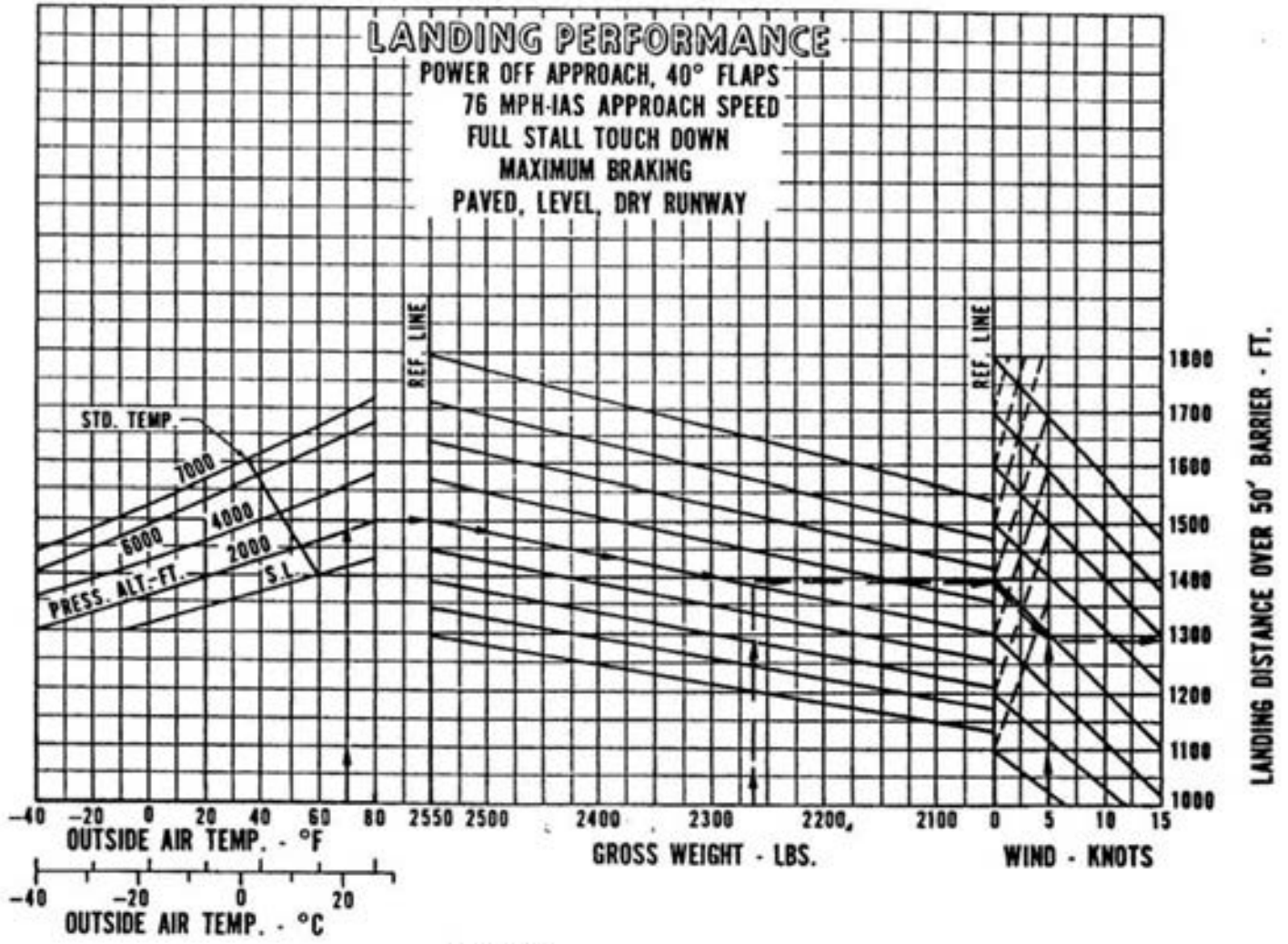
LANDING PERFORMANCE Figure 5-29
