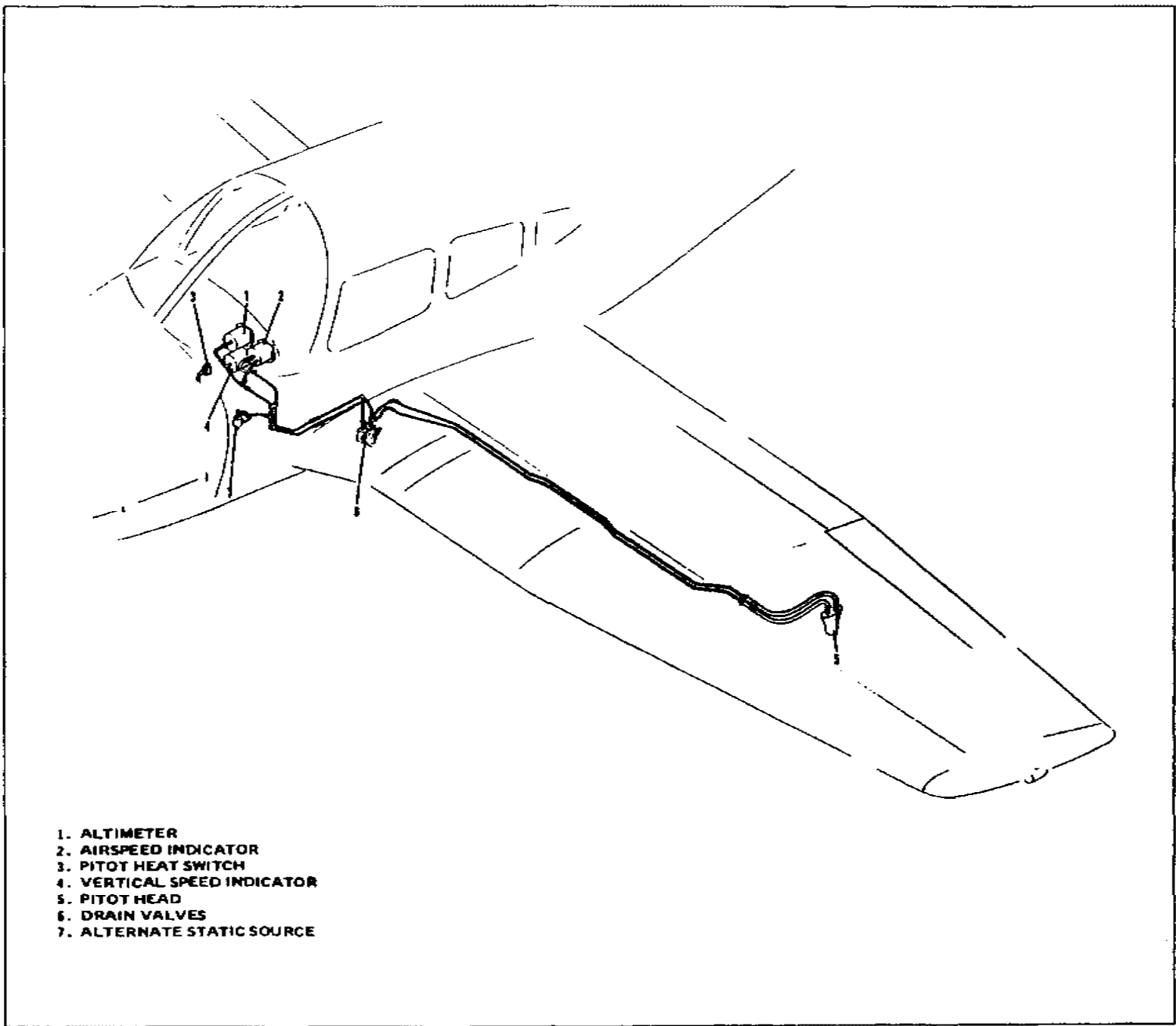
PITOT-STATIC SYSTEM
