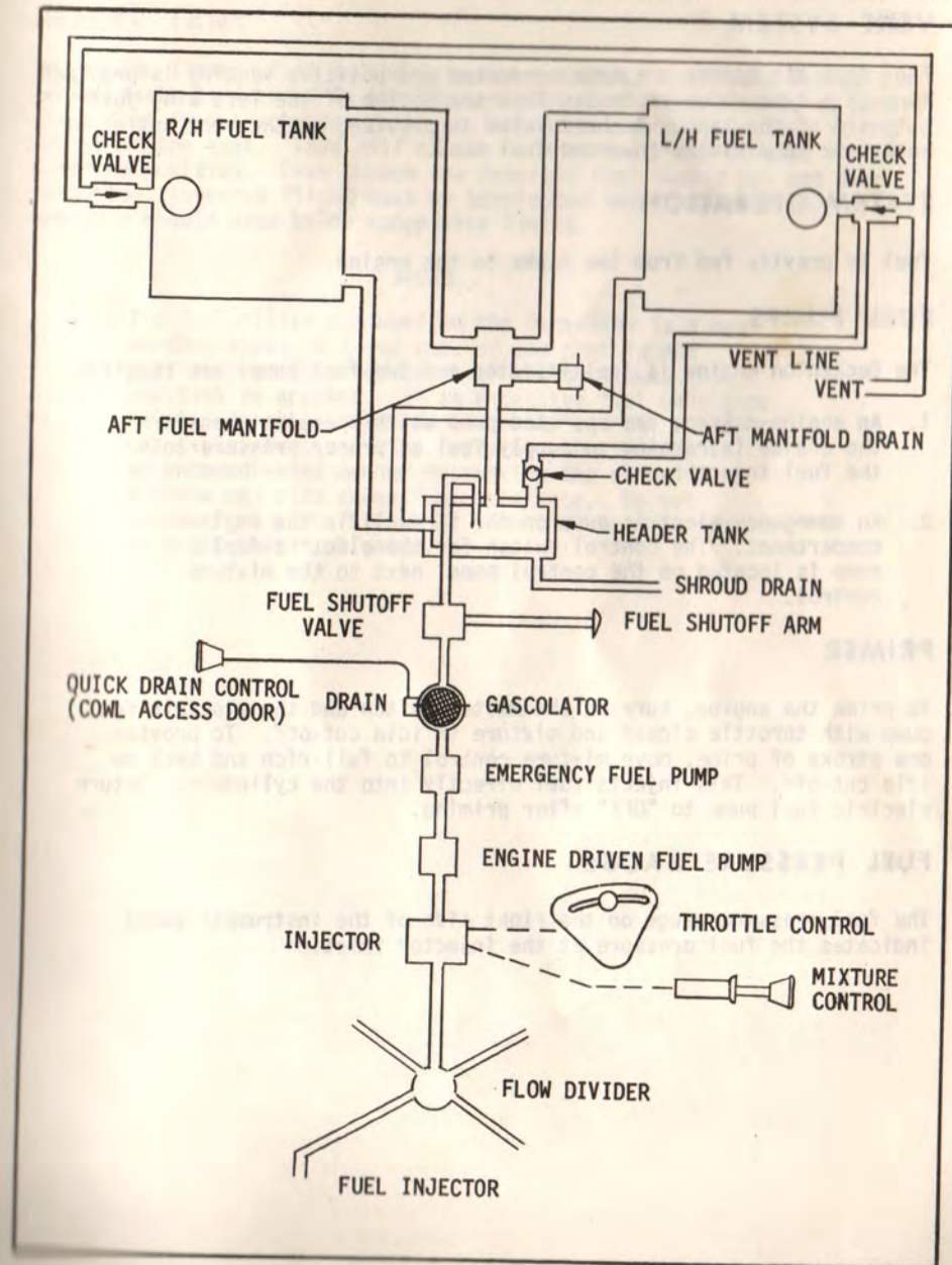
FIGURE 6-2 FUEL SYSTEM SCHEMATIC
