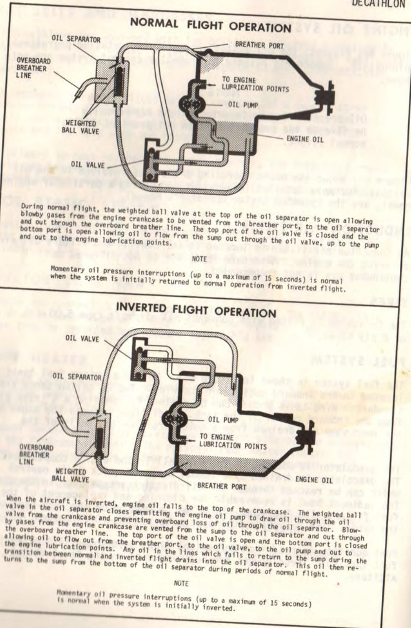
FIGURE 6-1 OIL SYSTEM SCHEMATIC
