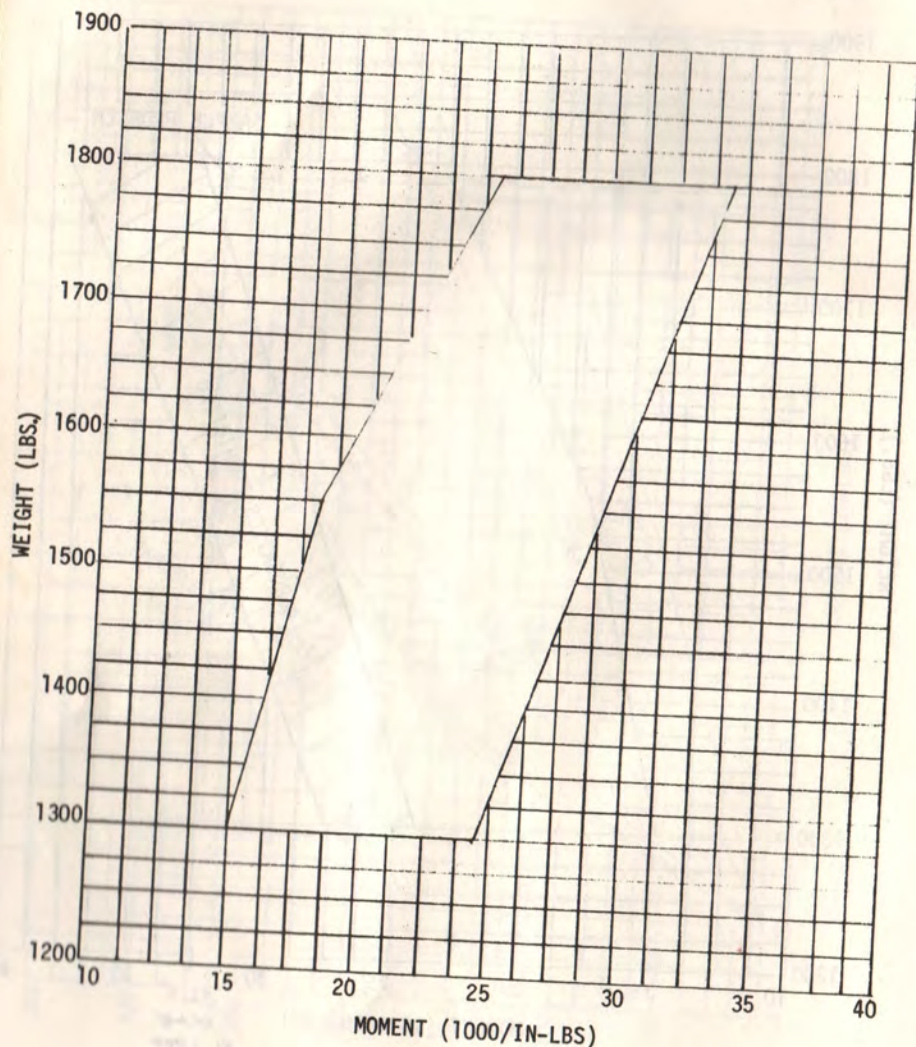
FIGURE 5-4 SUPER DECATHLON WEIGHT AND BALANCE FLIGHT ENVELOPE
