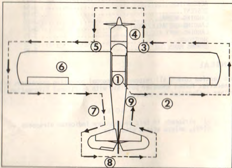
FIGURE 3-1 PREFLIGHT INSPECTION
