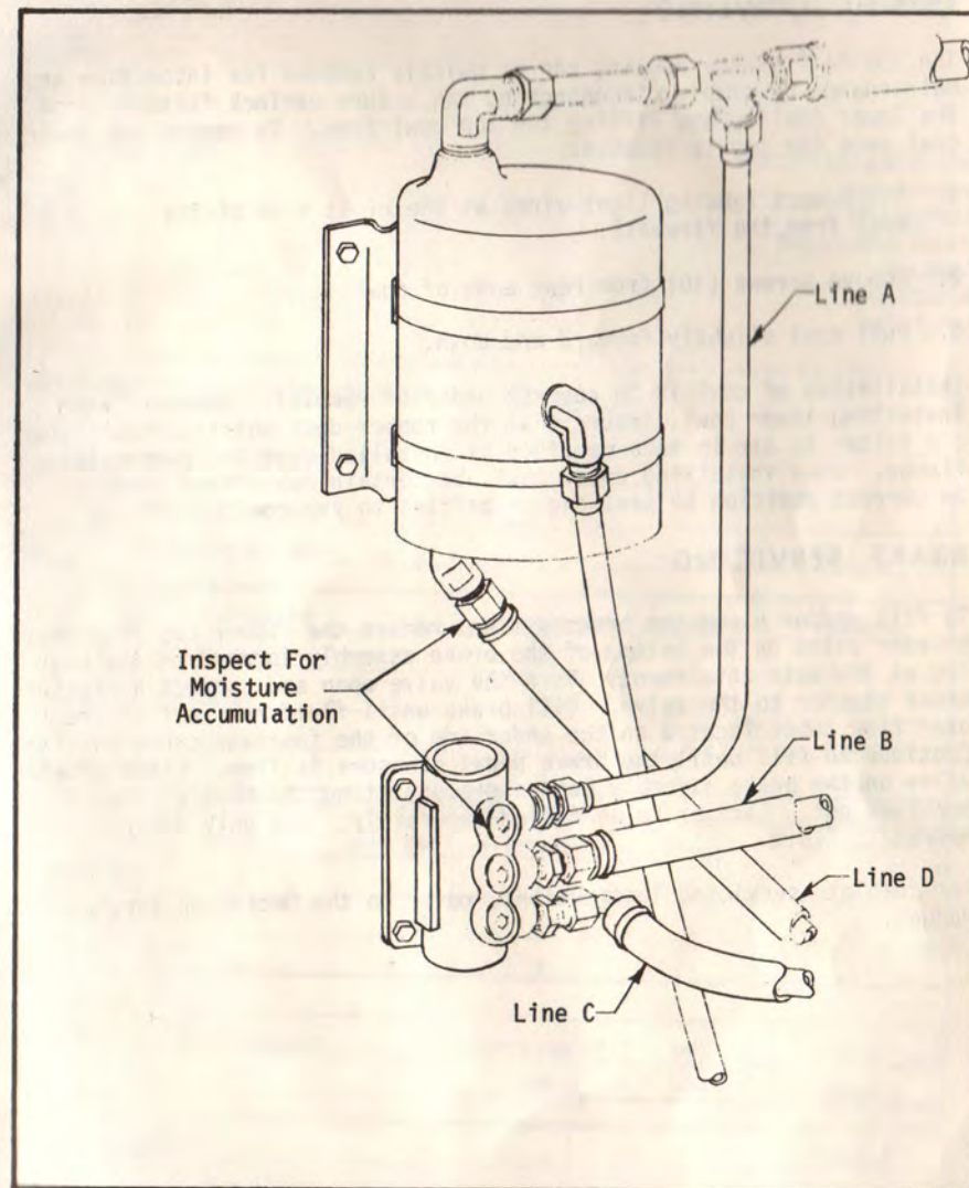
FIGURE 7-1 CHRISTEN OIL SYSTEM LINES AND INSPECTION POINTS
